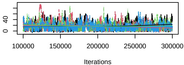
Trace of d.I.I_HER3i
