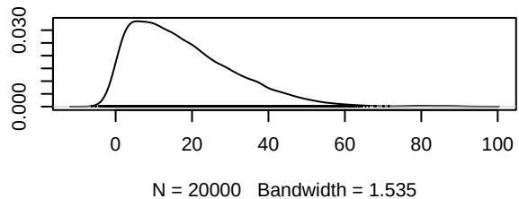
Density of d.I.I_HER3i
