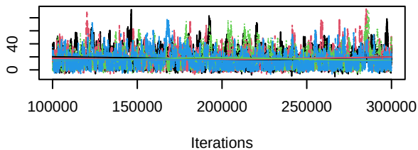
Trace of d.I.I_MMPi
