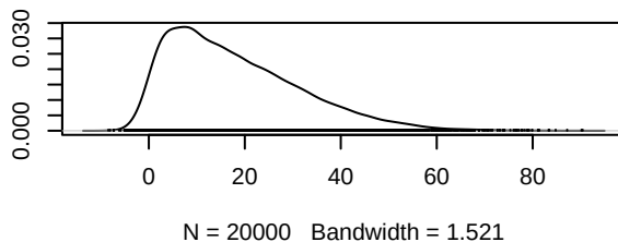
Density of d.I.I_PARPi
