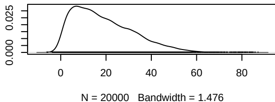
Density of d.III.III_antiangi
