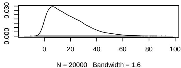
Density of d.I.I_MMPi
