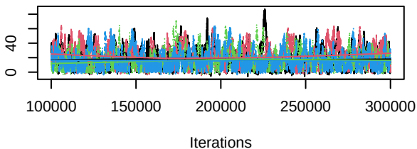
Trace of d.III.III_antiangi
