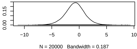
Density of d.III.III_Amivantamab
