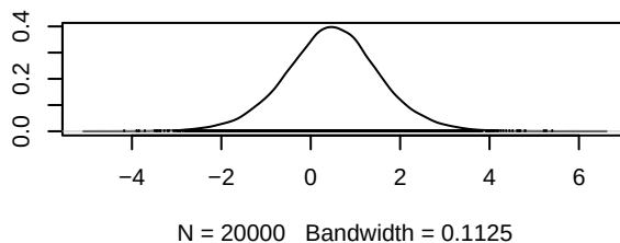
Density of d.I.III
