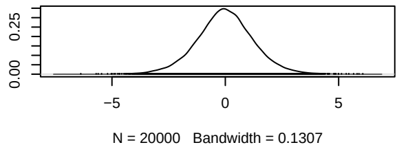
Density of d.I.I_METi
