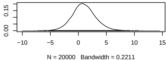
Density of d.I.I_IGF_1Ri
