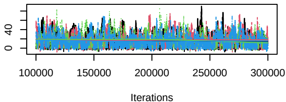
Trace of d.I.I_PARPi
